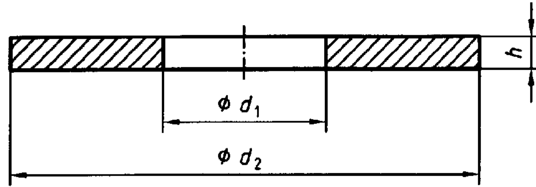
Figure 1 — Dimensions
